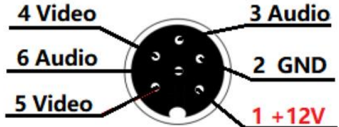
AV-IN 5~8 Camera Interface
