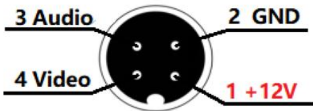
AV-OUT Display Interface
