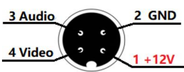
AV-IN 1~4 Camera Interface
